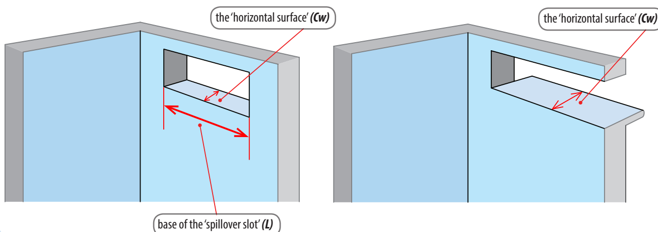
Figure 2 – Where to measure the 'horizontal surface' ( Cw ) and the base of the 'spillover slot' ( L )
